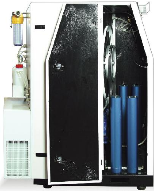
SCA400-PFS Purification Filter System with filters
