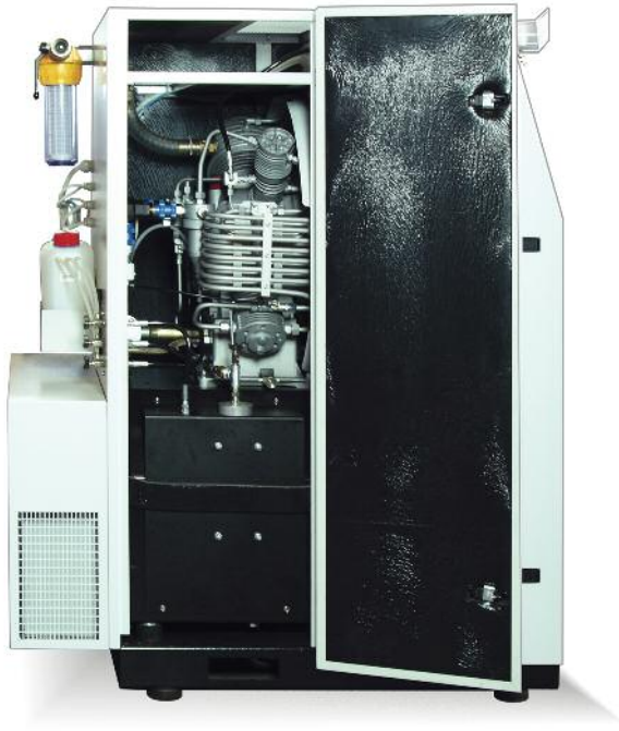
SCA400E43/CNG Block
